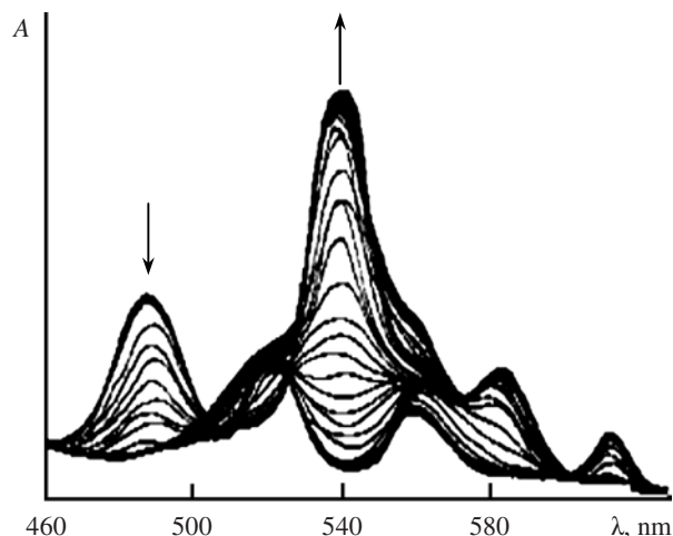
Fig. 4. Variations in the visible region of the electronic absorption spectrum of porphyrin VIII with decrease in pH (from 18 to 6) in the system \text{HClO}_4\text{--H}_2\text{O--MeCN} at 298 K ( c_{\text{VIII}} = 1.51 \times 10^{-5} M).
